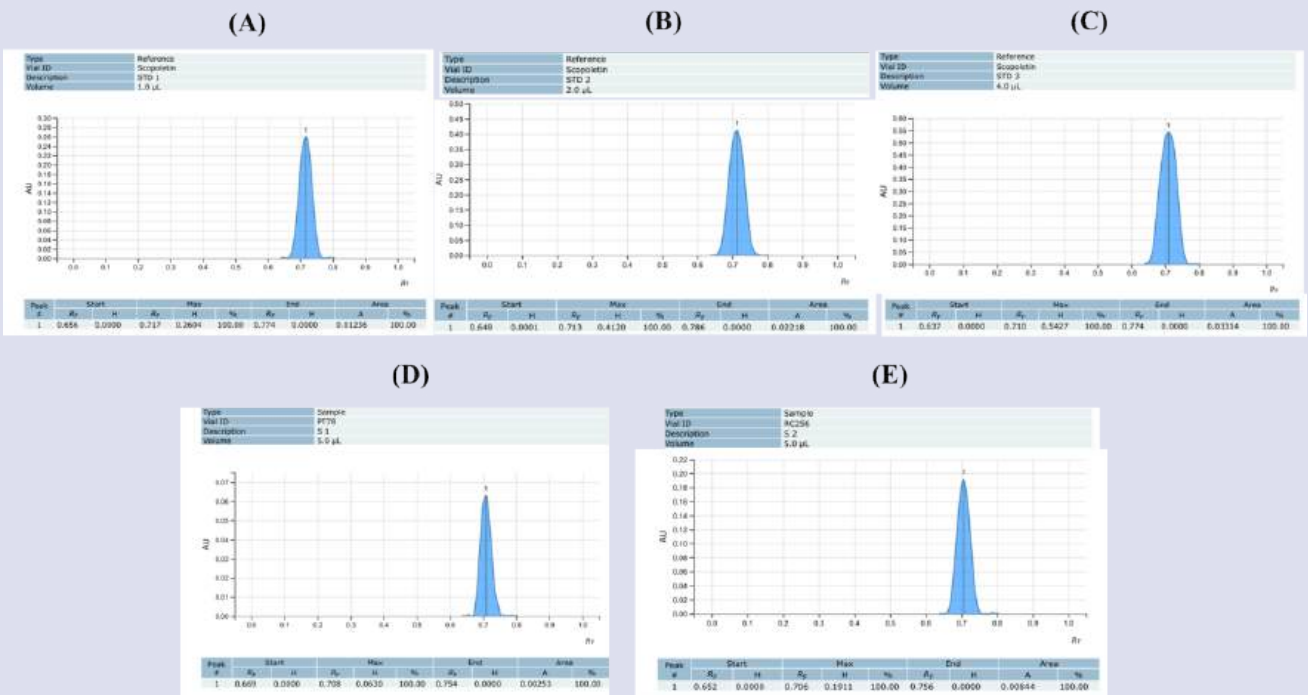
Figure 6. HPTLC chromatograms of [A] Scopeletin at 1.0 µL, [B] Scopeletin at 2.0 µL, [C] Scopeletin at 4.0 µL, [D] PT78 at 5.0 µL, and [E] RC256 at 5.0 µL using visionCATS software.
